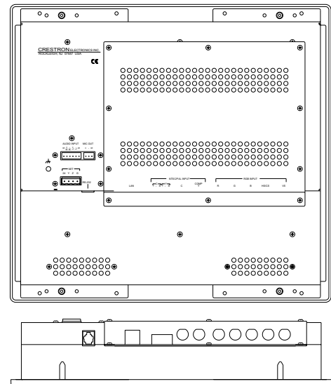
Isys TPS-6000L Bottom View
